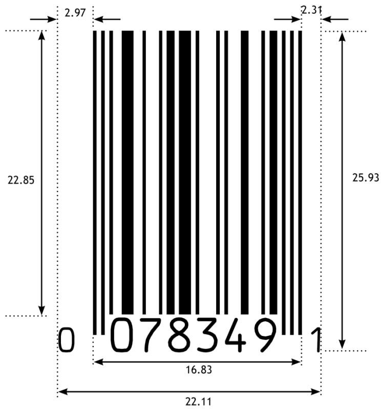
Figure 5.2.6.6-4. UPC-E barcode
