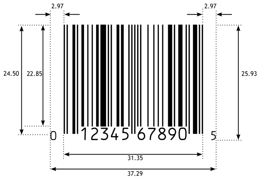
Figure 5.2.6.6-2. UPC-A barcode
